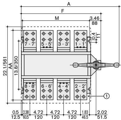
1. Terminal screen
