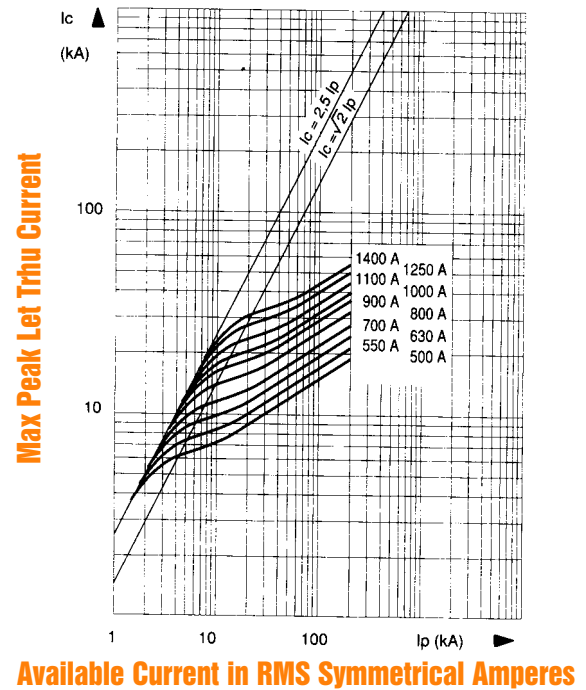
Peak Let-Thru Current Data
