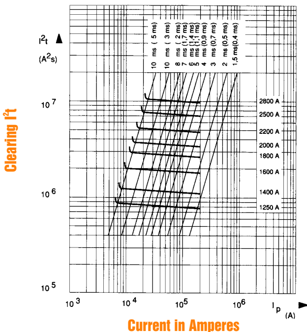
Clearing I^2t Data 2X33
