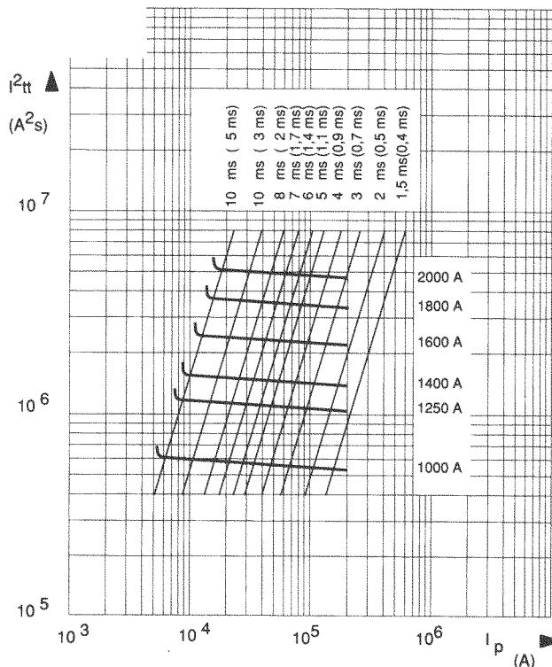
Clearing I 2 t Data 2X32
