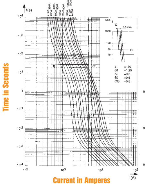
Melting Time – Current Data
