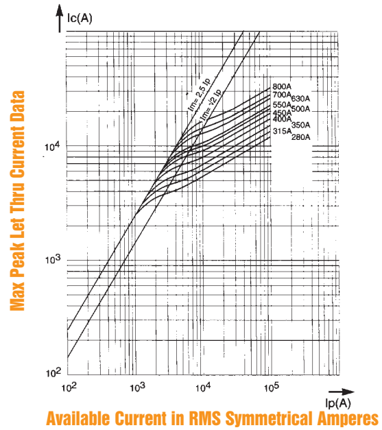
Peak Let-Through Current Data
