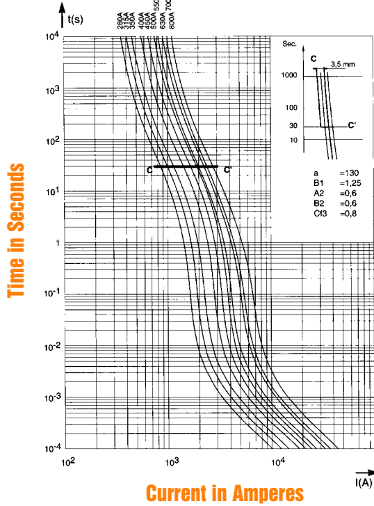
Melting Time — Current Data
