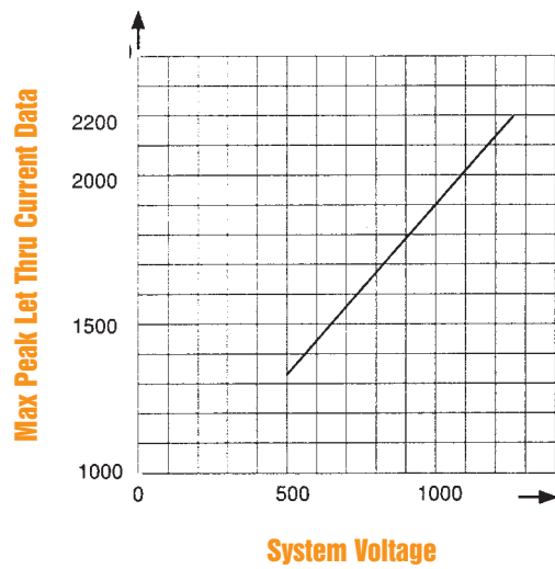
Maximum Arc Voltage vs. System Voltage
