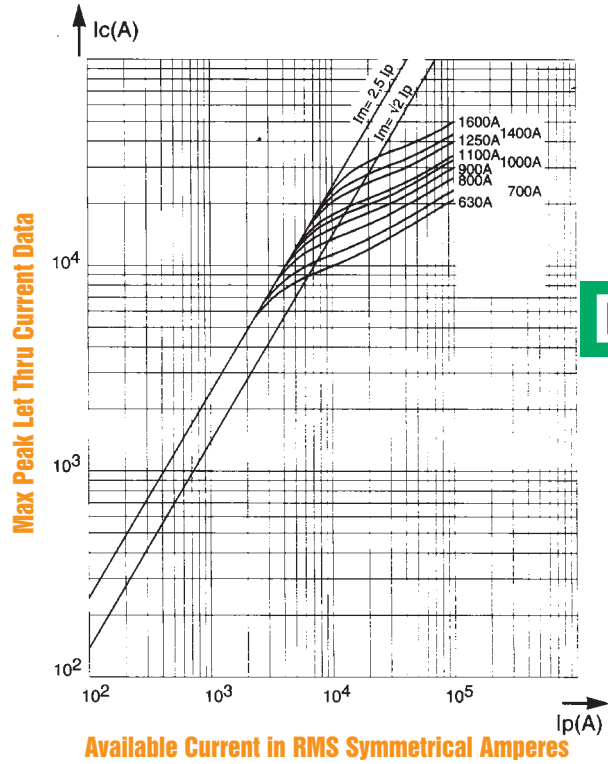
Peak let thru Current Data
