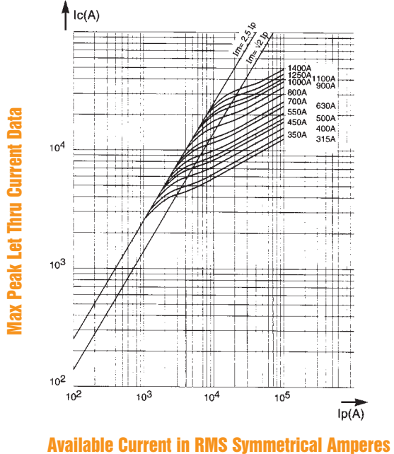
Peak Let-Through Current Data
