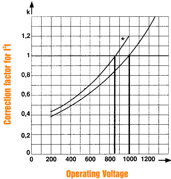
Clearing I 2 t vs. Operating Voltage
