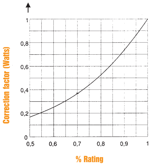
Watts Loss vs. Rated Current
