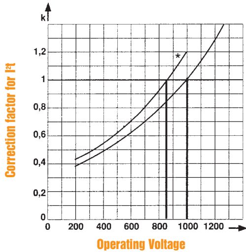
Clearing I 2 t vs. Operating Voltage
