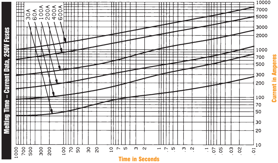
A2K30 to 600
