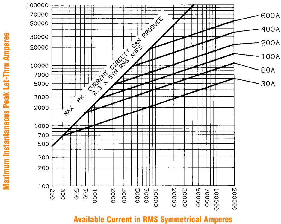
Peak Let-Thru Current Data — 30 to 600, 600 Volts AC
