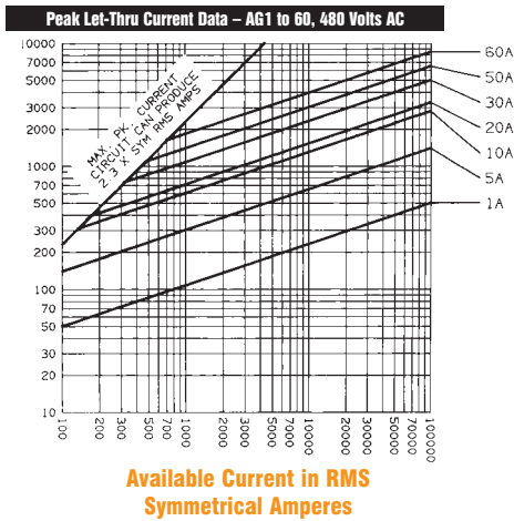
Maximum Instantaneous Peak Let-Thru Amperes
