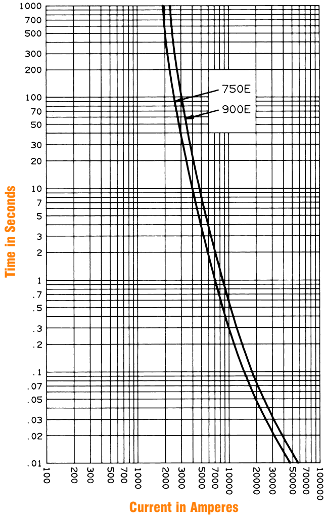
Minimum Melting Time — Current Data, 5.5kV Fuses
