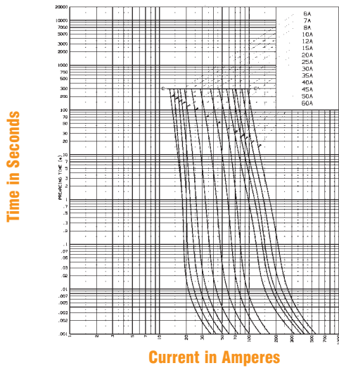
Melting Time - Current Data A30QS 1 to 60
