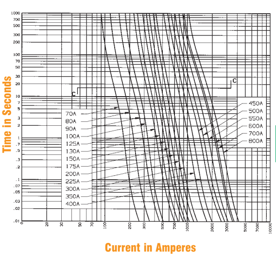
Melting Time - Current Data A30QS 70 to 800
