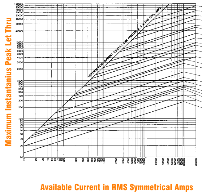
Peak Let Thru Data
