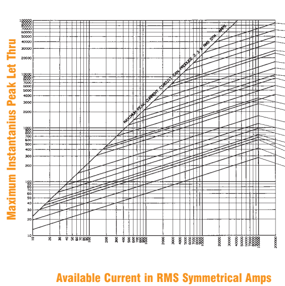
Peak Let Thru Data
