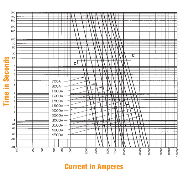
Melting Time - Current Data A30QS 700 to 4500
