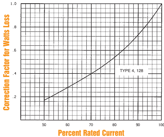
Watts loss vs. Percent Rated Current
