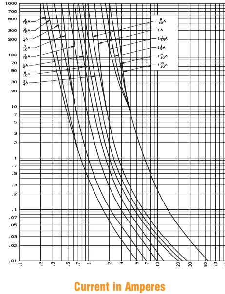
Melting Time-Current Data ATQR 3/16 to 1-8/10, 600 Volts
