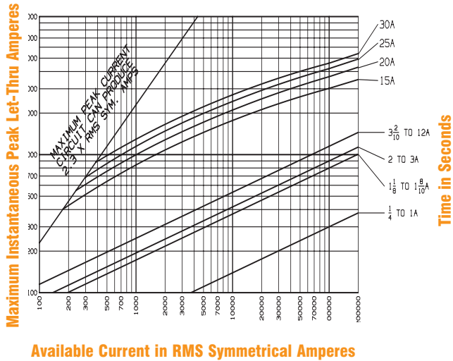
Peak Let-Thru Current Data—ATQR1/4 to 30, 600 Volts AC
