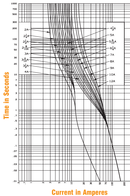
Melting Time-Current Data ATQR 2 to 30, 600 Volts AC
